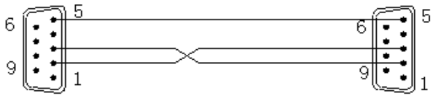
DB9 pins of the port
