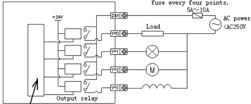
Relay output circuit
